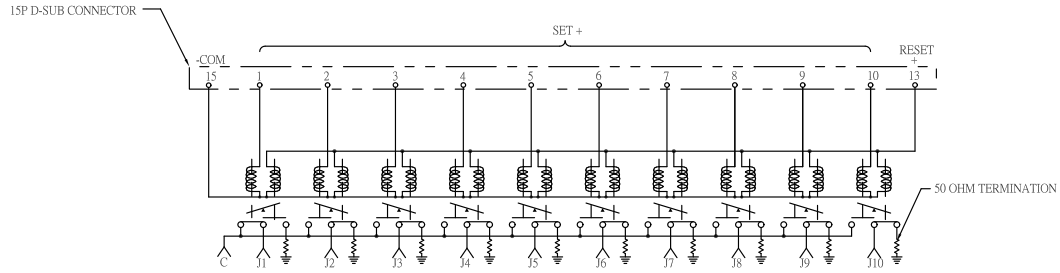
SCHEMATIC COIL I SHOWN LAST ENERGIZE
