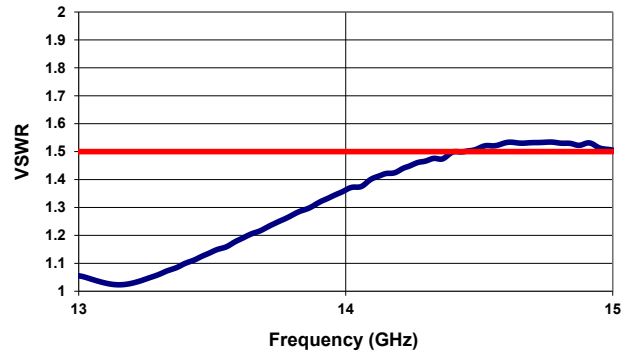
VSWR ( 13-15 GHz )
