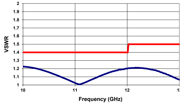
VSWR ( 10-13 GHz )
