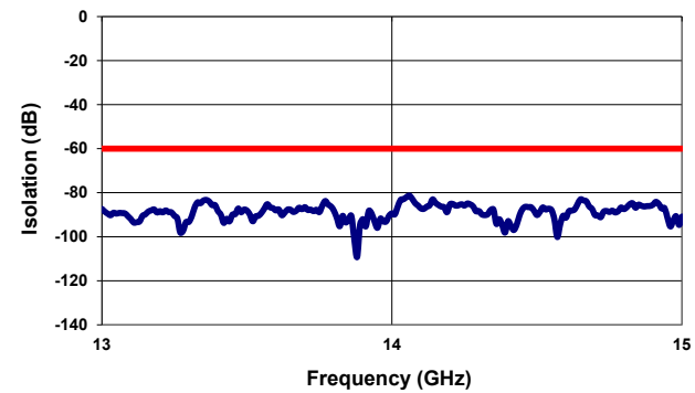
Isolation ( 13-15 GHz )
