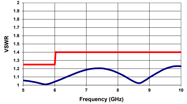
VSWR ( 5-10 GHz )
