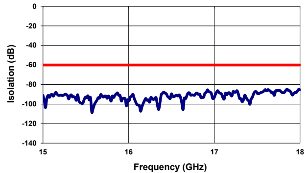
Isolation ( 15-18 GHz )
