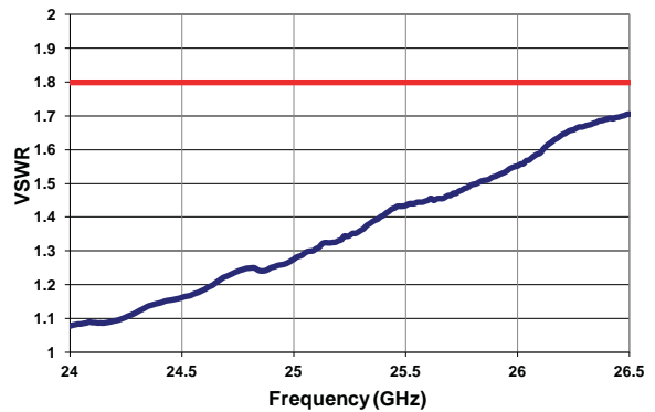
VSWR ( 24-26.5 GHz )
