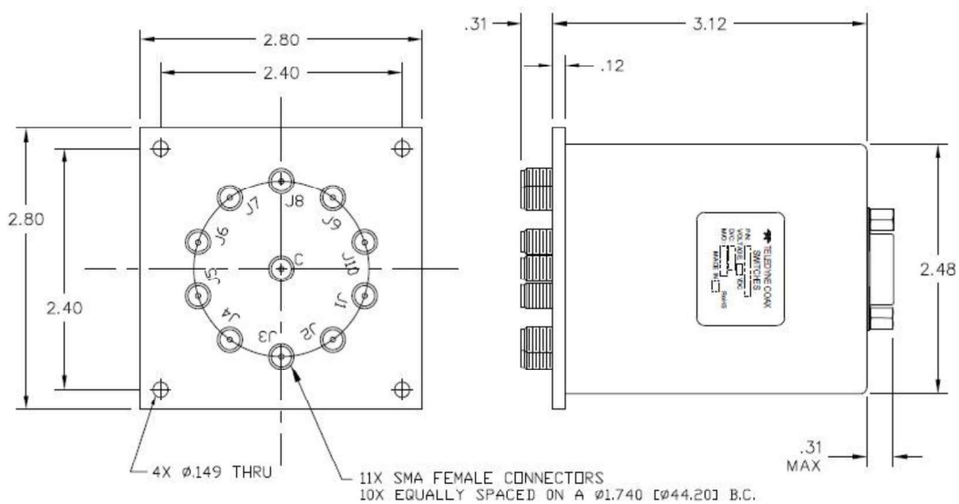
“-TS OR -TDS OPTIONS” 15-PIN D-SUB OR 25-PIN D-SUB CONNECTOR (EXAMPLE: CCR-38S180-TS OR CCR-38S180-TDS)
