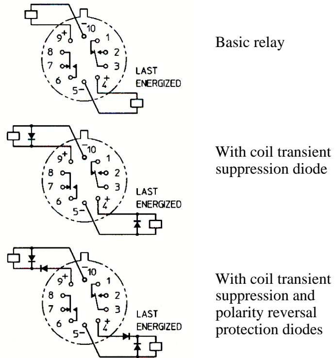
Figure 2. Terminal locations and circuit diagram (bottom view).
