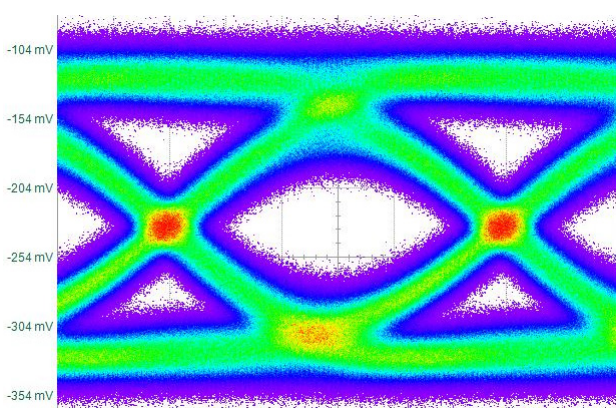
InP1012-60 @ 48 Gbps
