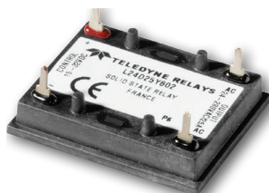
L Series Single Phase AC 25A, 280Vac Ultraminiature SSR
