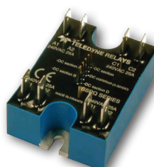
SQ Series Quad Output SSR 25A, 280Vac each
