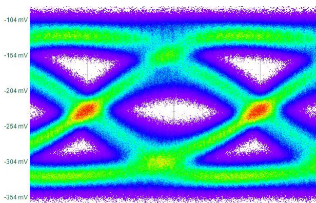
InP1012-60 @ 56 Gbps
