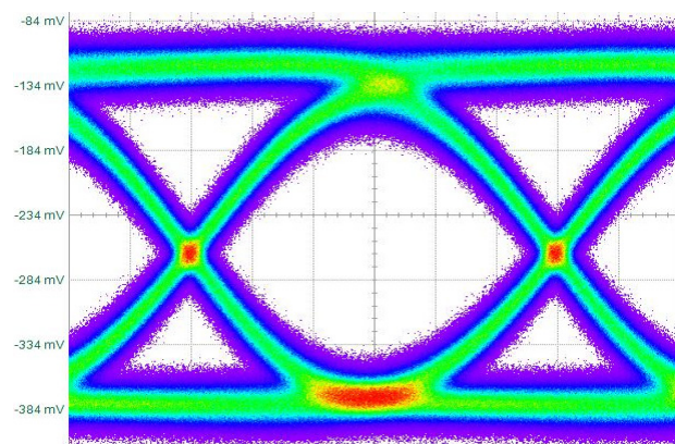
Reference @ 48 Gbps
