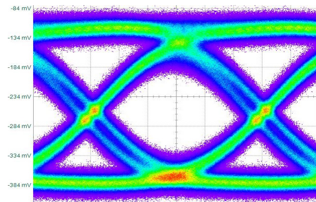
Reference @ 56 Gbps
