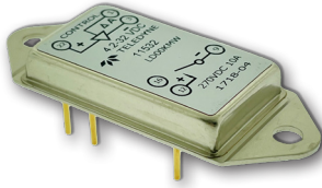
LD00KM 10A, 270Vdc Load 4.2-32Vdc Control
