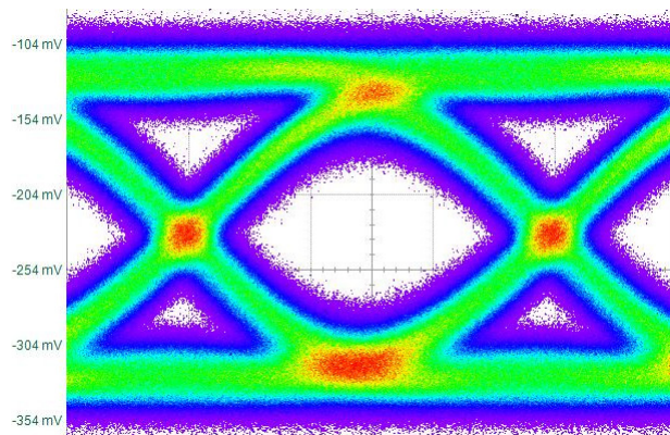
InP1012-60 @ 40 Gbps
