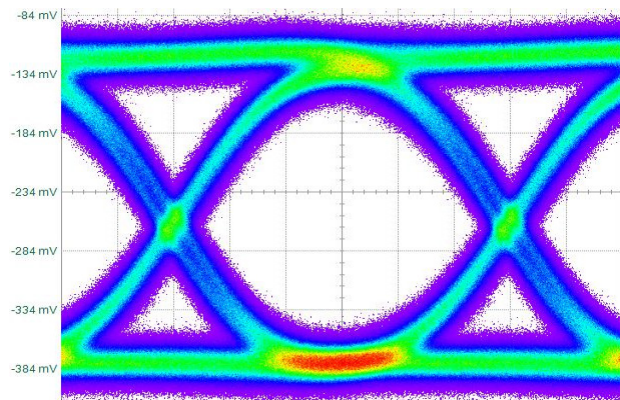
Reference @ 40 Gbps
