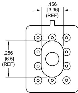
“M9”Spacer Pad for Centigrad®
