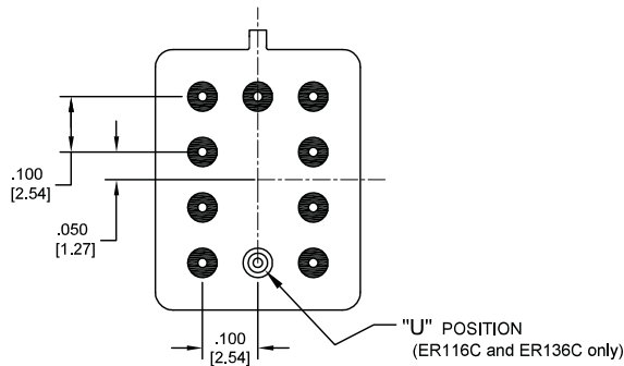
Centigrad® Relays: RF180, ER116C, 122C, ER136C
