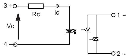
Figure 3 — LS relays
