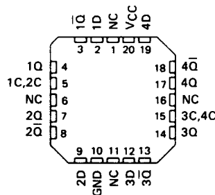
SN54LS375 . . . FK PACKAGE (TOP VIEW)
