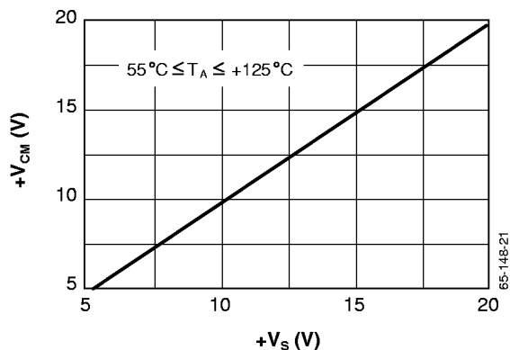
Figure 19. Positive Common Mode, Input Voltage vs. Supply Voltage
