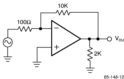
Figure 10. Gain, Phase Test Circuit
