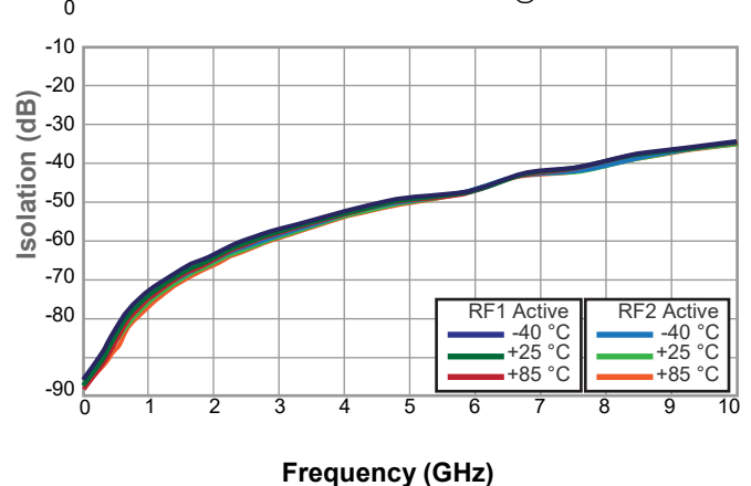
PE95421 Isolation RF1-RF2 @ 3.3V
