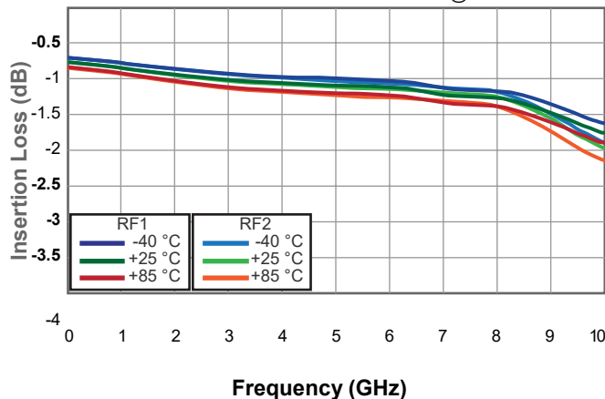
PE95421 Insertion Loss RF1 and RF2 @ 3.3V
