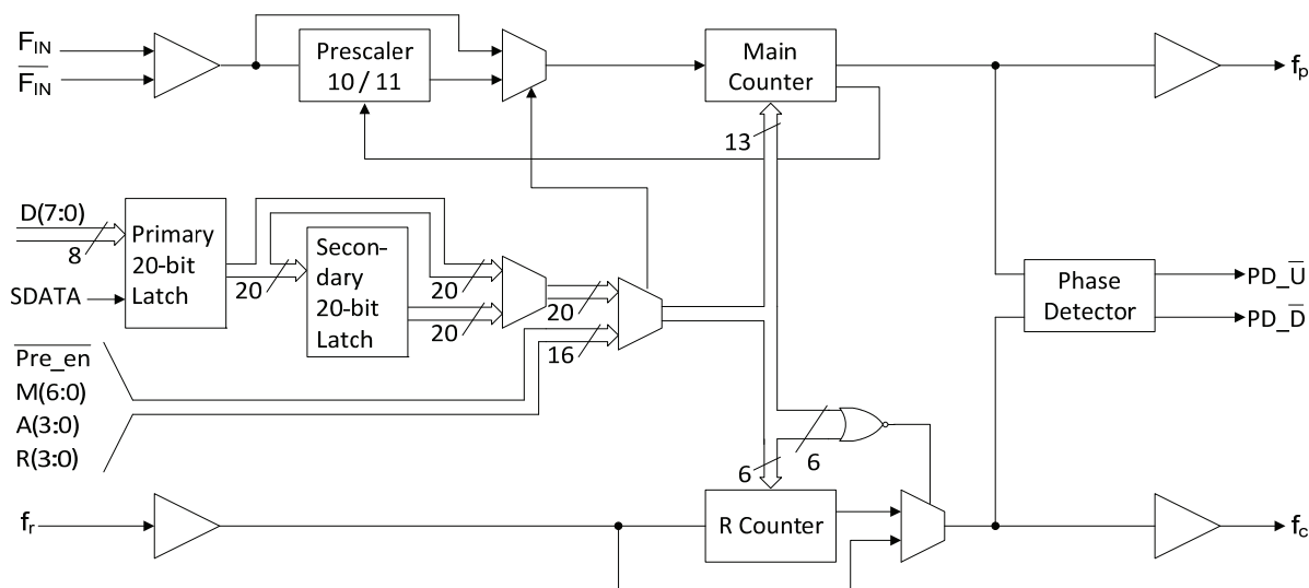
Figure 1. Block Diagram
