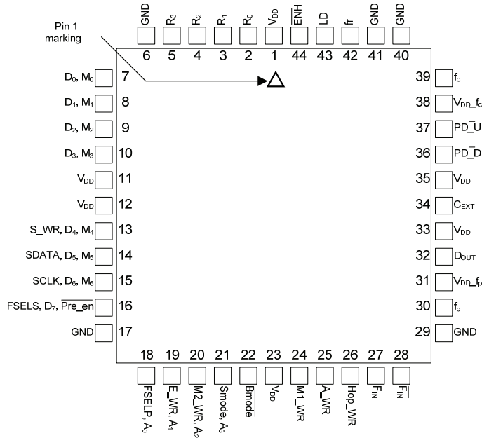
Figure 2. Pin Configuration (Top View)
