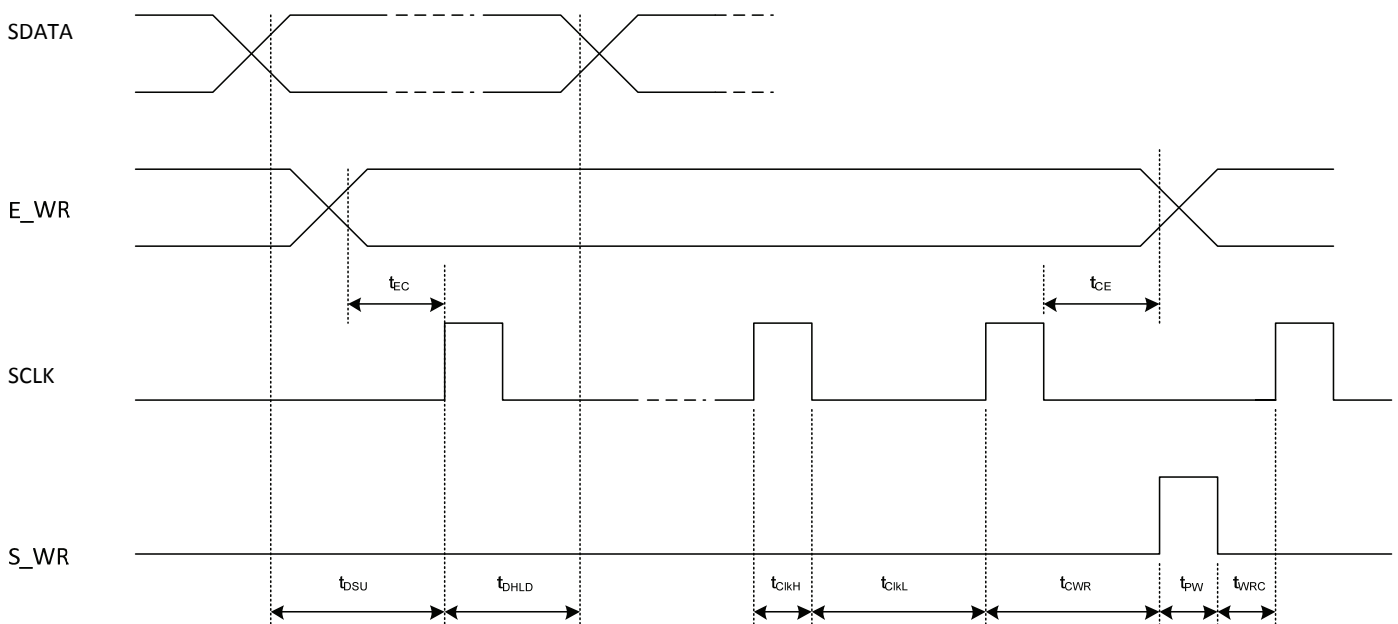
Figure 11. Serial Interface Mode Timing Diagram
