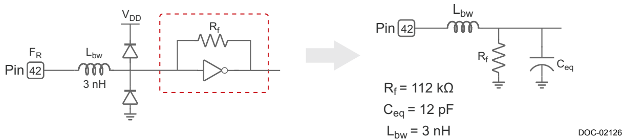
Figure 7. Equivalent Input Diagram: Reference Input
