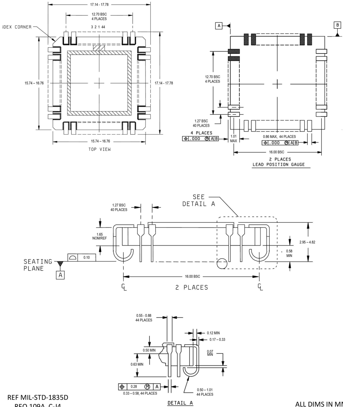
Figure 12. Package Drawing (dimensions are in millimeters) 44-lead CQFJ
