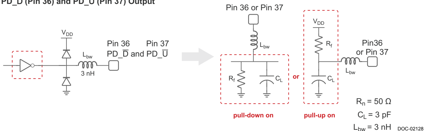
Figure 9. Equivalent Output Diagram: PD \bar{D} & PD \bar{U} Outputs
