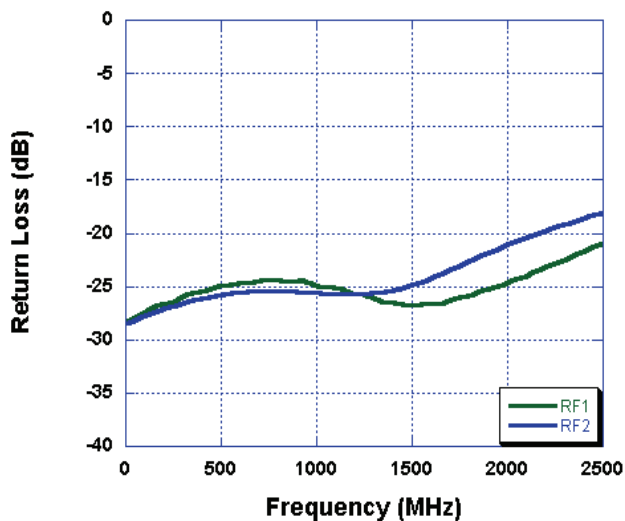
Figure 11. Return Loss – RF1, RF2
