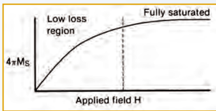
Figure 4 4\pi M_s vs Applied Field
