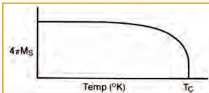
Figure 5 Effect on 4\pi M_s as Temperature is raised
