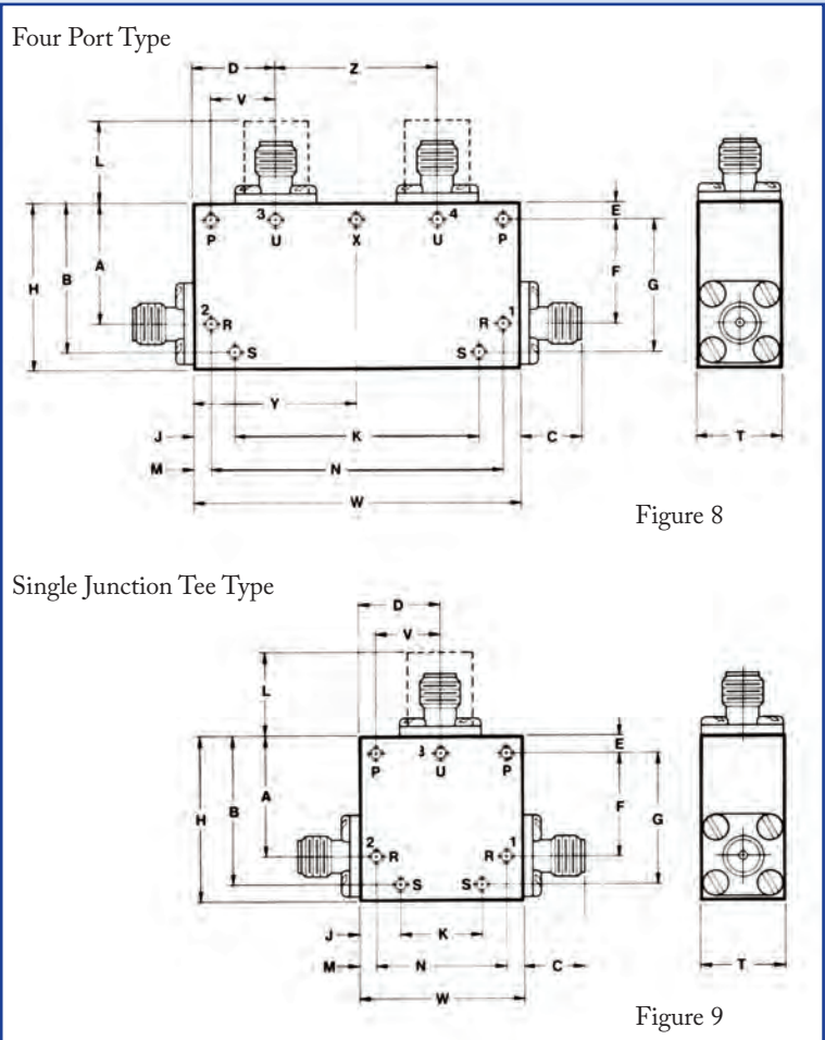
Several mounting options are provided. For specific models, use these drawings for reference and consult the factory, or ask for a mechanical outline drawing.
