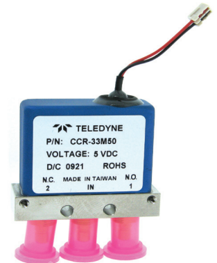
DC Flying Leads
