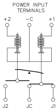
SCHEMATIC
