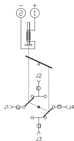
SCHEMATIC
