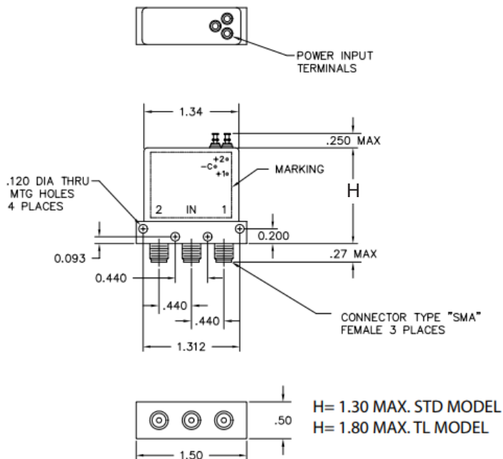
Standard Width Body
