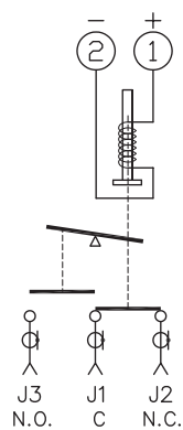
SCHEMATIC
