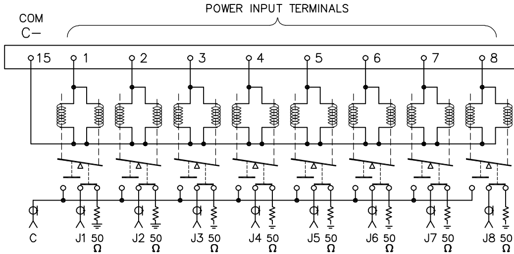
SP8T Failsafe (N.O.) - Terminated
