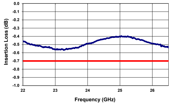
Insertion Loss ( 22-26.5 GHz )
