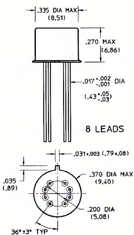
Figure 1. Outline dimensions.
