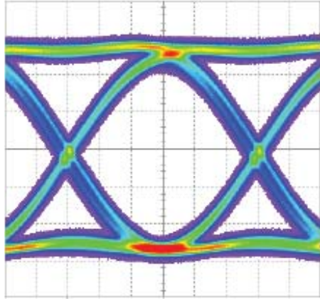
Reference @ 40Gbps
