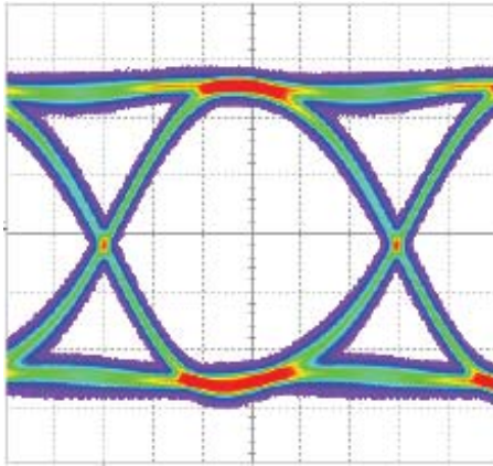
GRF121 @ 16Gbps
