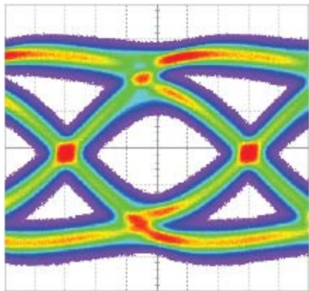
GRF121 @ 40Gbps
