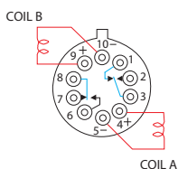
SCHEMATIC (Coil A Last Energized) (Bottom View)
