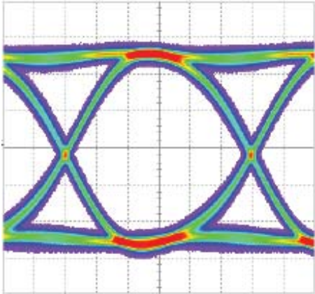
GRF121 @ 16Gbps
