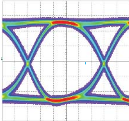
Reference @ 16Gbps
