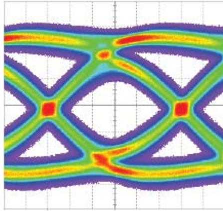
GRF121 @ 40Gbps
