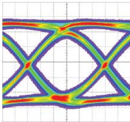
Reference @ 28Gbps
