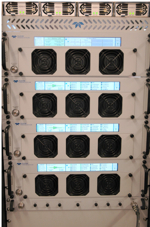
PowerMAX System with 4 SSPA Modules
