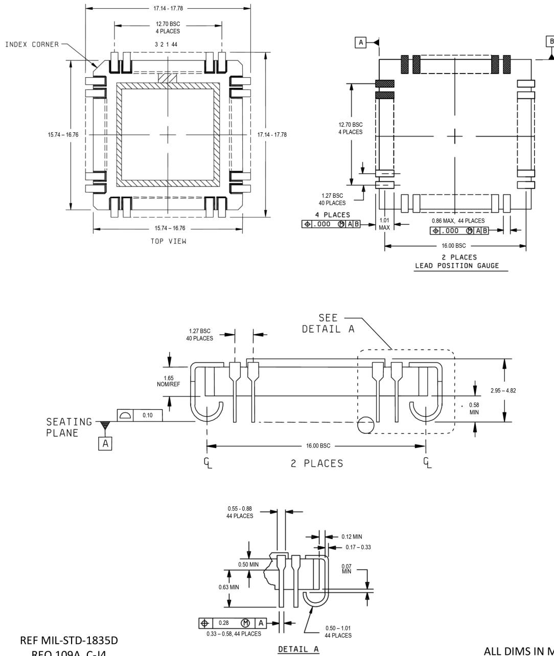
Figure 7. Package Drawing 44-lead CQFJ
