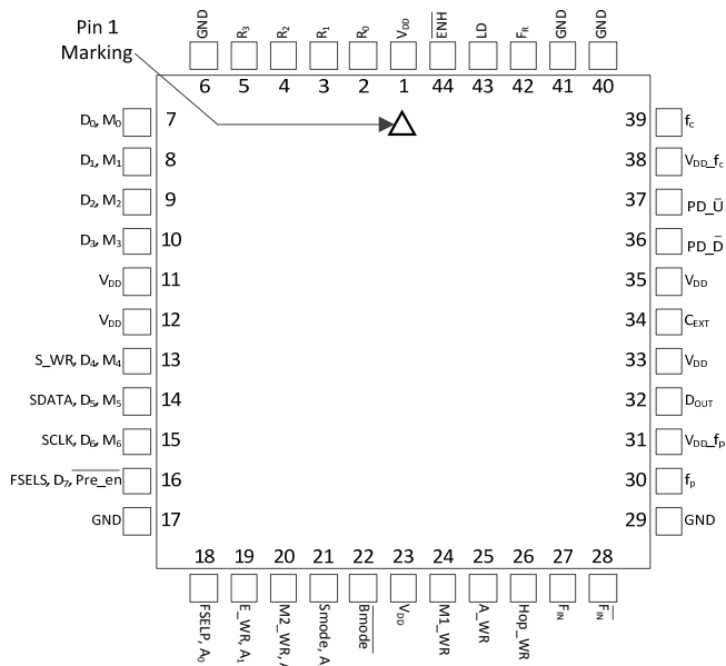
Figure 2. Pin Configuration (Top View)
